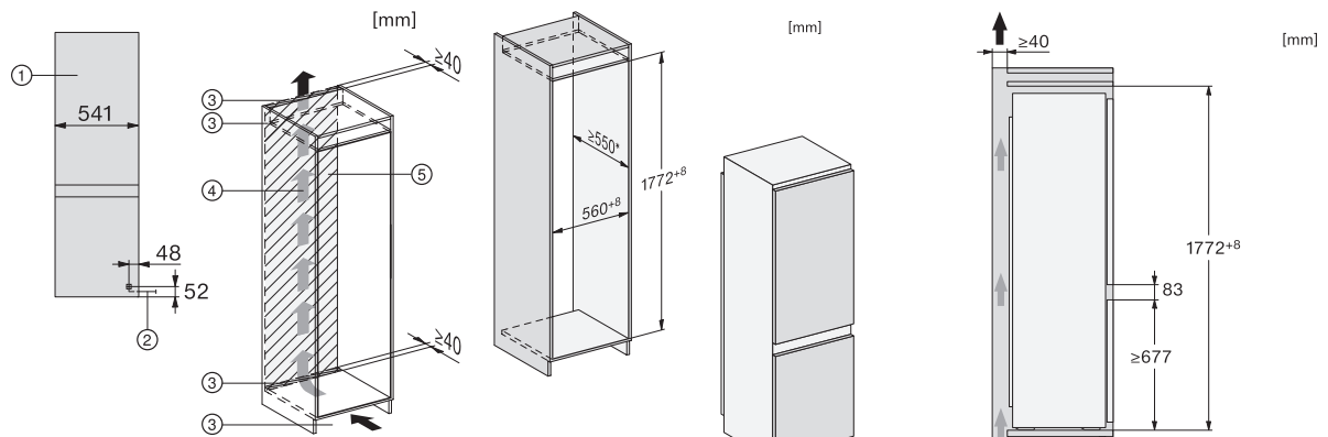
KD7713E, KD7714E, KD7724E, KDN7713E, KDN7714E, KDN7724E Active, installation (footnote*) (installation drawings)
