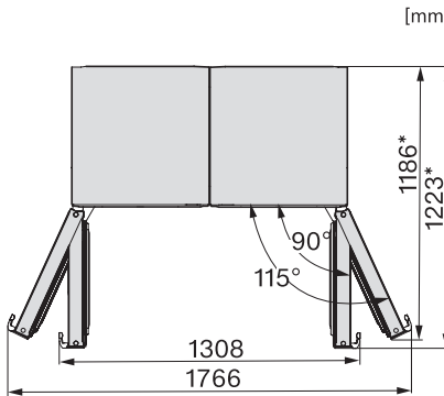
FNS4782E, FNS4782E N, FNS4882D N, top view (footnote*) (installation drawings)
