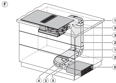
KMDA 7633, KMDA 7634, KMDA 7476 - built-in version 7 (Installation drawing)
