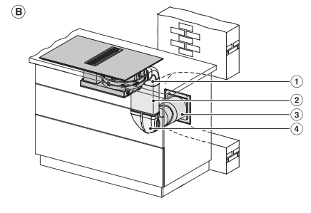
KMDA 7633, KMDA 7634, KMDA 7476 - Built-in version 6 (Installation drawing)
