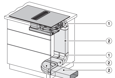
KMDA 7633, KMDA 7634, KMDA 7476 - built-in version 7 (Installation drawing)
