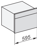
DGC7x4x, DGC7x4xX, DGC7x4xHCPro, DGC7x4xHCXPro installation drawings
