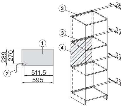
DG7x40, DGC7x4x, DGC7x6x, DG7635, DGM7x4x, DO7, H2860B/BP, H7240BM, H7x40BM, H7x4xB/BP, H7x6xB/BP, installation drawings
