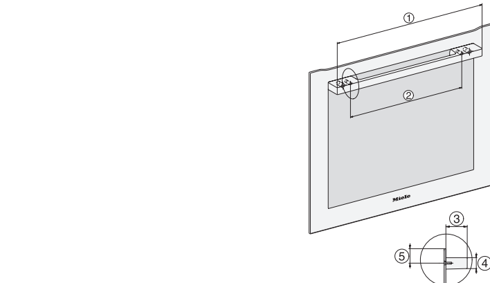
H2x6x-1B/BP/E/EP/I/IP, H2850BP, H7x6xB/BP/BPX, H2x6xB, installation drawings
