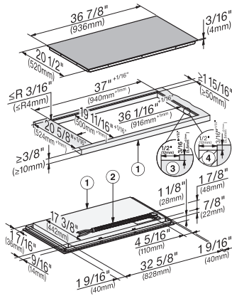
KM7747FL Diamond – flush installation – drawing
