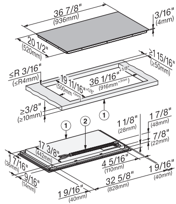
KM7747FL Diamond – frameless overlying installation
