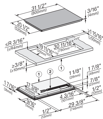
KM7737FL Diamond – frameless overlaying installation
