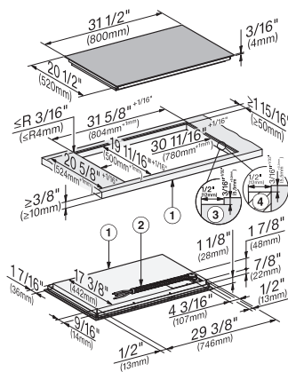
KM7737FL Diamond – flush installation – drawing
