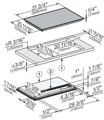
KM7737FR Diamond – frameless overlaying installation
