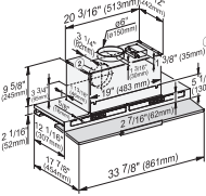
DAS8930, drawing – US
