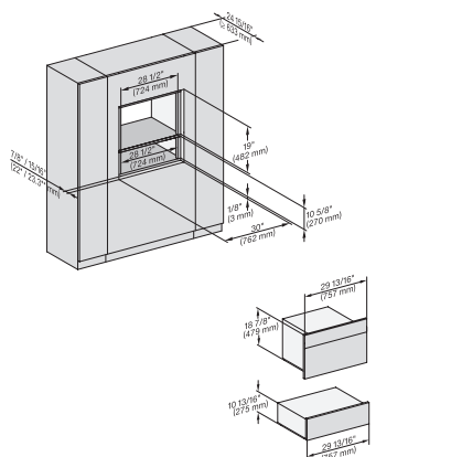
H 6x70 BM, ESW 6x80, DGC 7xxx, H7x70 BM/BMX, ESW 7x80 Fitting Combi wide front, Installation drawing, Flush inset, NA
