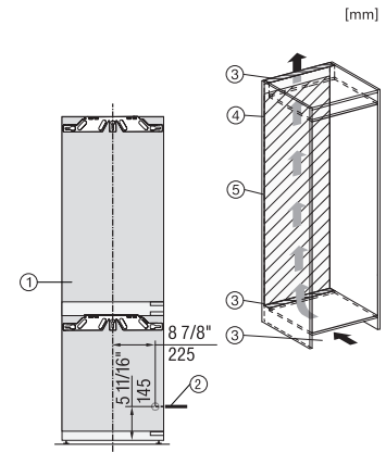
KFN7734D, KFN7734C, KFN7784D, installation (US)
