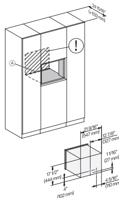
CVA7445, CVA7845, installation drawing, 60 cm, Flush inset
