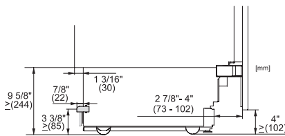
36inch, connection for power/water supply, MasterCool (US, CA, MX) (Sketch)
