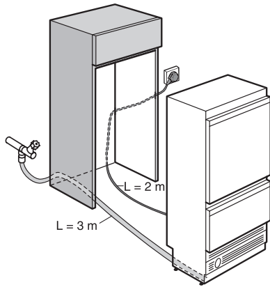
laying cabling and pipework, MasterCool (installation drawings)
