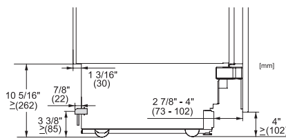
18 inch, connection for power/water supply, MasterCool (US, CA, MX) (Sketch)
