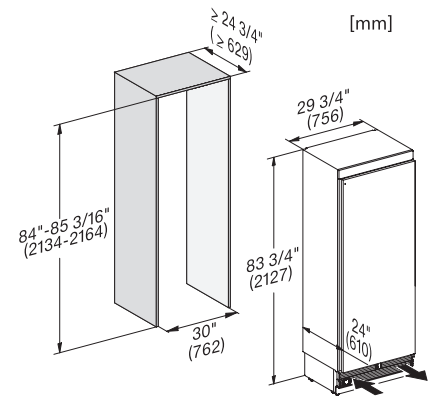
F2812Vi, F2813Vi, F2802Vi, F2811Vi, F2801Vi, MasterCool, inner space, installation drawings
