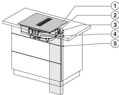
KMDA5649FL, KMDA5649FR, KMDA5649FL MattFinish – Installation variant 1 Basis
