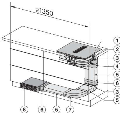
KMDA5649FL, KMDA5649FR, KMDA5649FL MattFinish – Installation variant 5 Circulating air
