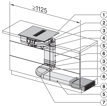
KMDA5649FL, KMDA5649FR, KMDA5649FL MattFinish – Installation variant 13 Circulating air
