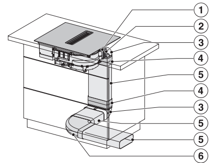
KMDA5649FL, KMDA5649FR, KMDA5649FL MattFinish – Installation variant 3 Basis
