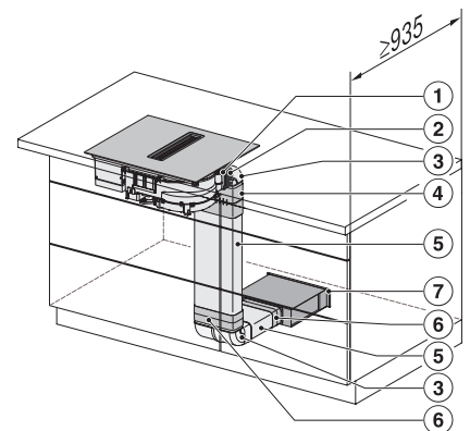
KMDA5649FL, KMDA5649FR, KMDA5649FL MattFinish – Installation variant 6 Circulating air
