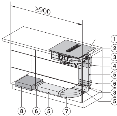
KMDA5649FL, KMDA5649FR, KMDA5649FL MattFinish – Installation variant 14 Circulating air
