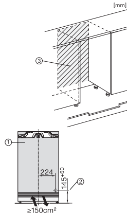
KU7016D, KU7015D, KU7035D, KU7135C, FNUS7140C, Built-under, installation drawing (*footnote)
