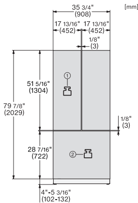
KFMC3642FD, KFMC3844FD, MasterCool III, front view (*Footnote) (installation drawing) (US)
