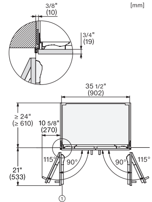
KFMC3642FD, KFMC3844FD, MasterCool III, PACS, with stainless steel front, top view (installation drawing) (US)
