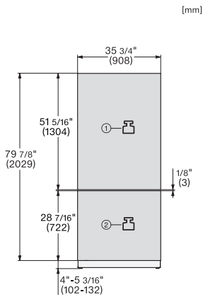
KFMC3642R, KFMC3842L, KFMC3844R, KFMC3844L, MasterCool III, front view (*Footnote) (installation drawing) (US)
