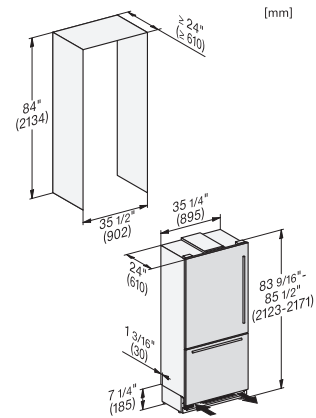
KFMC3642R, KFMC3642L, KFMC3844R, KFMC3844L, MasterCool III, PACS, with stainless steel front, integration (drawing)
