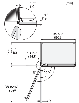
KFMC3642R, KFMC3642L, KFMC3844R, KFMC3844L, MasterCool III, PACS, with stainless steel front, top view (drawing) (US)
