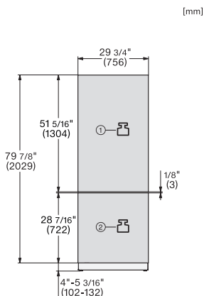
KFMC3632R+L, KFMC3836R+L, KFMC3834R+L, MasterCool III, front view, installation (*Footnote) (drawing)
