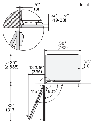
KFMC3632R+L, KFMC3836R+L, KFMC3834R+L, MasterCool III, panel ready, top view (drawing) (US)
