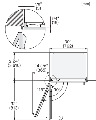
KFMC3632R+L, KFMC3836R+L, KFMC3834R+L, MasterCool III, PACS, with stainless steel front, top view (drawing) (US)
