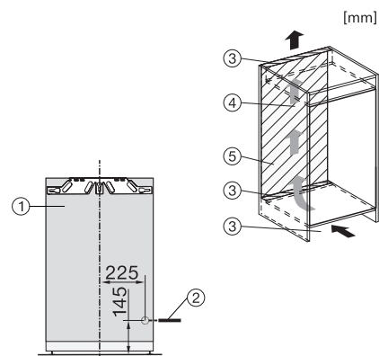
FNS7140B, FNS7140C, FNS7140D, FNS7140E, installation (*footnote) (installation drawings)
