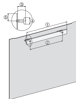
H226x-1B/BP/E/EP/I/IP, H24xx installation drawings
