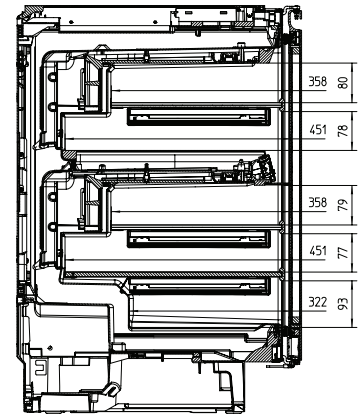
KWT6321UG, Interior dimensions (Installation drawings)
