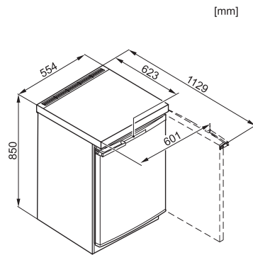
F12011S, F12011S-1 F12011S-2 (installation drawings)
