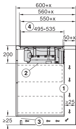
KMDA7272-1FL, KMDA7473-1FL, KMDA7272FL, KMDA7473FL – Side view flush+X, Plug&Play
