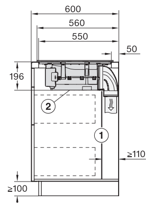
KMDA7272-1FL, KMDA7473-1FL, KMDA7272FL, KMDA7473FL – Side view lying on top
