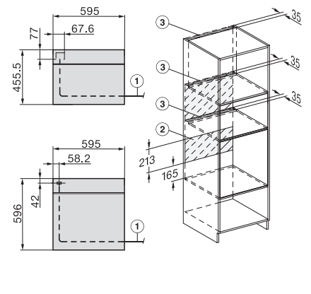
Installation Kombi BM XL, installation drawings 22 mm – glass, 23.3 mm – metal
