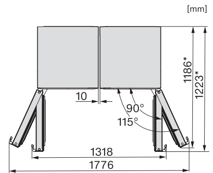
KS4783DD, KS4783ED, FNS4782E, FNS4782D, top view, Side-by-Side (*footnote) (installation drawings)
