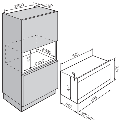
H 5981 BP, H 6890 BP - 90 cm (Installation drawing)
