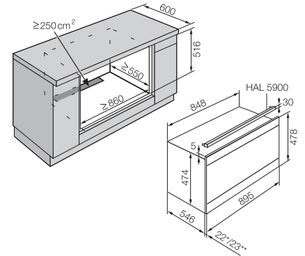
H 5981 BP, H 6890 BP - 90 cm (Installation drawing)
