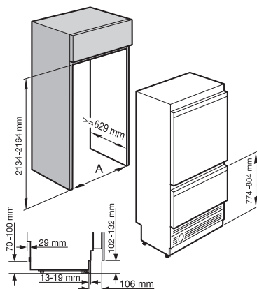
KF1801Vi, KF1811Vi, KF1901Vi, KF1911Vi, dimensions of appliance, MasterCool (Sketch) *Footnote
