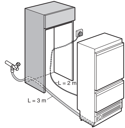
laying cabling and pipework, MasterCool (installation drawings)
