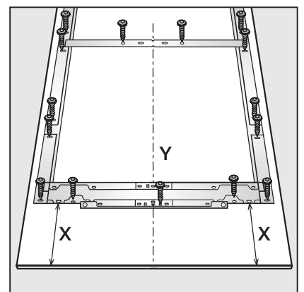
K1801Vi, K1901Vi, KF1801Vi, KF1901Vi, F1411Vi, F1811Vi, F1911Vi, securing fixing frame, MasterCool (Sketch) *Footnote
