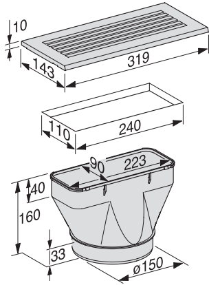
DUU151 (installation drawing)
