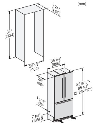
KFMC3642FD, KFMC3844FD, MasterCool III, PACS, with stainless steel front, integration (installation drawing)
