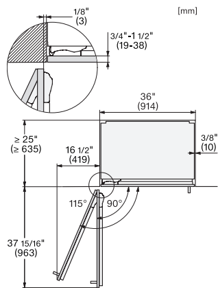
KFMC3642R, KFMC3642L, KFMC3844R, KFMC3844L, MasterCool III, panel ready, top view (installation drawing) (US)
