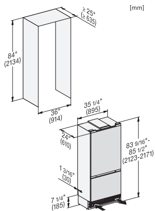
KFMC3642R, KFMC3842L, KFMC3844R, KFMC3844L, MasterCool III, integration, panel ready (installation drawing) (US)
