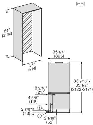
KFMC3642R, KFMC3842L, KFMC3844R, KFMC3844L, MasterCool III, installation, panel ready (installation drawing) (US)
