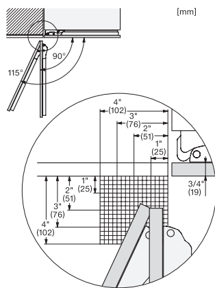
KFMC3632R+L, KFMC3642R+L, KFMC3836R+L, KFMC3834R+L, KFMC3858FD, MasterCool III, hinge clearance, installation (drawing)
