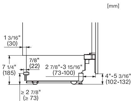
KFMC3642R, KFMC3842L, KFMC3844R, KFMC3844L, MasterCool III, front view (*Footnote) (installation drawing) (US)
