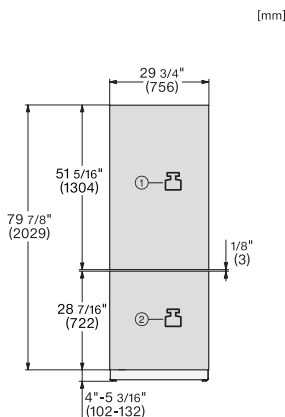
KFMC3632R+L, KFMC3836R+L, KFMC3834R+L, MasterCool III, front view, installation (*Footnote) (drawing)
