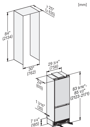
KFMC3632R+L, KFMC3836R+L, KFMC3834R+L, MasterCool III, integration, panel ready (installation drawing) (US)
