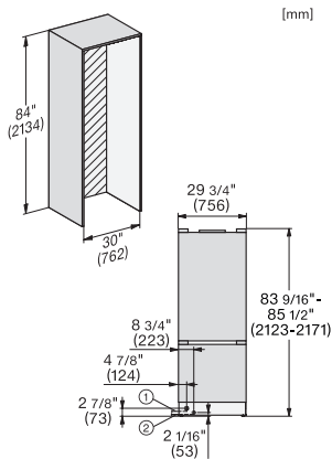
KFMC3632R+L, KFMC3836R+L, KFMC3834R+L, MasterCool III, installation, panel ready (*Footnote) (drawing) (US)
