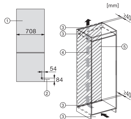
KFN7934D, installation
