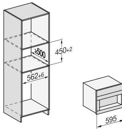
CVA7000 (installation drawings)
