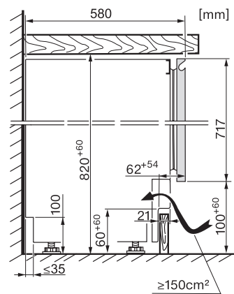
KWTUS7054F, KWTUS7055F, KWTUS7074F, Built-under, side view (installation drawings)
