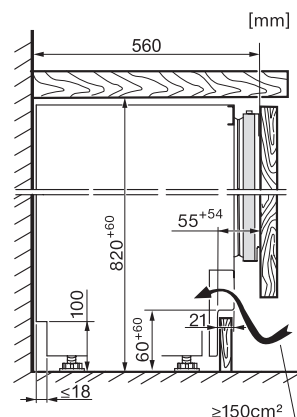
KU7016D, KU7015D, KU7035D, FNUS7040D, Built-under, side view (installation drawings)
