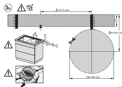
KMDA7272FL/FR, KMDA7473FL/FR – Installation variant 14 Circulating air – drawing
