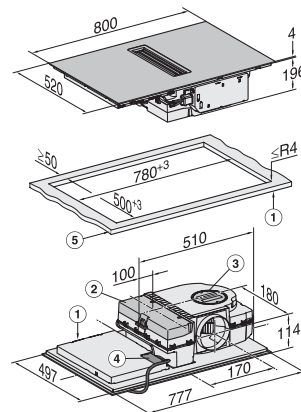
KMDA7272FL, KMDA7473FL – Installation drawing
