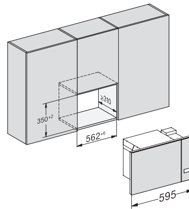
M223xSC, installation drawings
