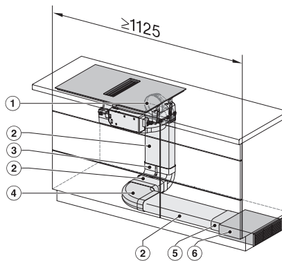
KMDA7676-1FL, KMDA7876-1FL, KMDA7676FL, KMDA7876FL – Installation variant 13 Circulating air
