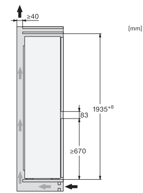
KFN7913E, side view
