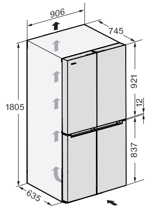
E-Com, KFFD6741 edt/cs, installation diagram
