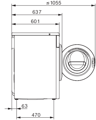
WT1 8/5 kg, drawing, straight facia, measures in mm
