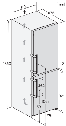
KFN4777CD, installation sketch
