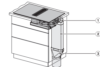
KMDA 7633, KMDA 7634, KMDA 7476 - built-in version 8 (Installation drawing)
