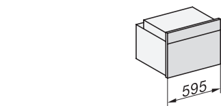
built-in H7000 M build-under, installation drawing
